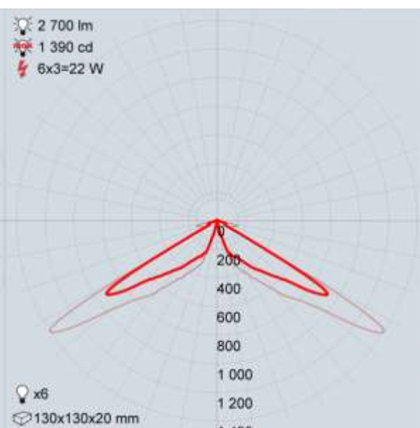
RefLED/.../60D
