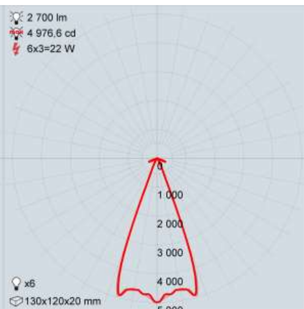
RefLED/.../20D
